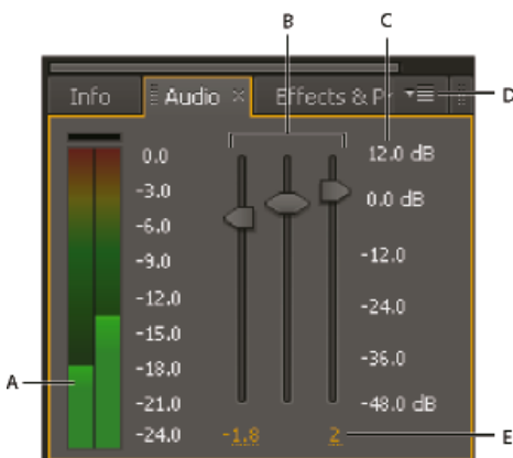
Audiofenster
